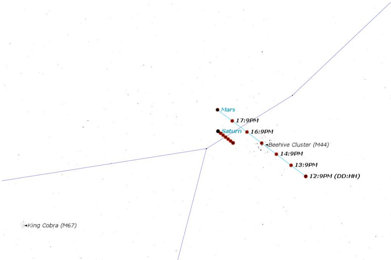
Mars crosses the Beehive Cluster June 12 to 18
